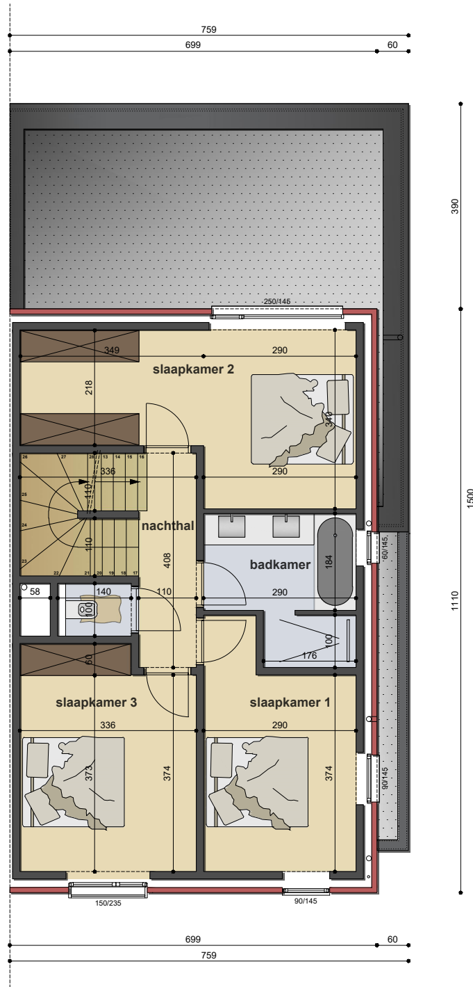
VERDIEPING 1 LOT 4
